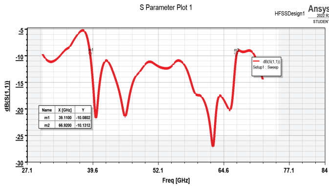
Fig. 14. Return loss characteristic using Split Ring Resonator With increased substrate height
