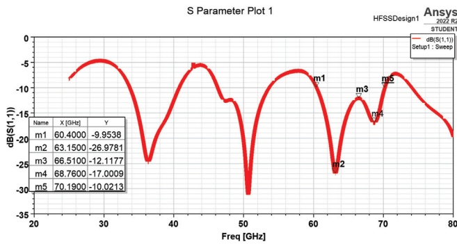
Fig. 6. S11 parameter of the proposed design2
