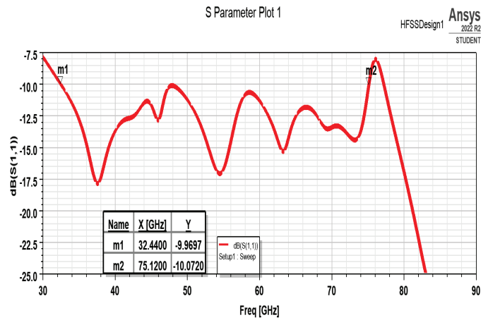
Fig. 9. Increased substrate height
