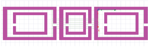
Fig. 11. Multi Split Ring Resonator
